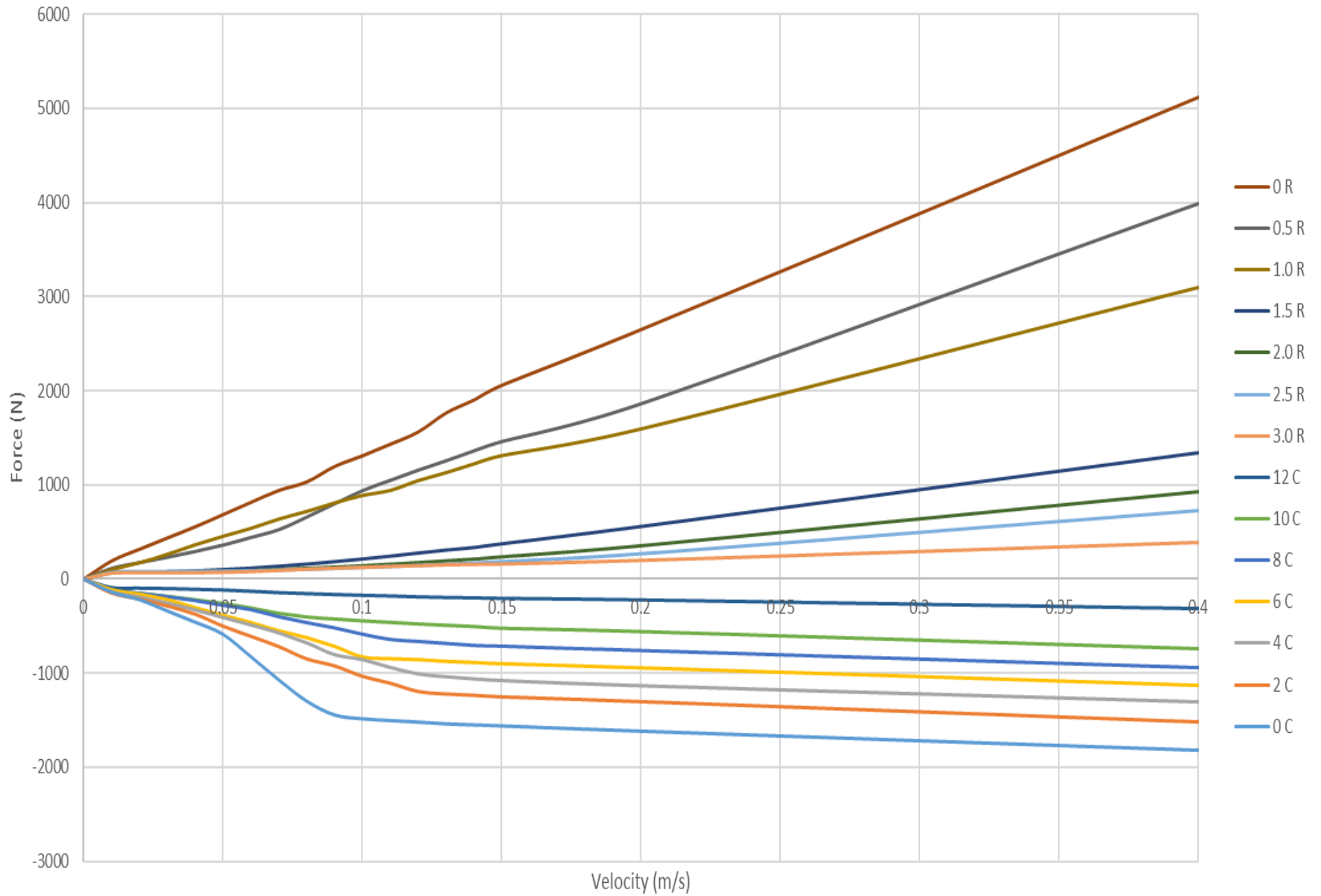
50th Anniversary CJ Front Damper Curves
