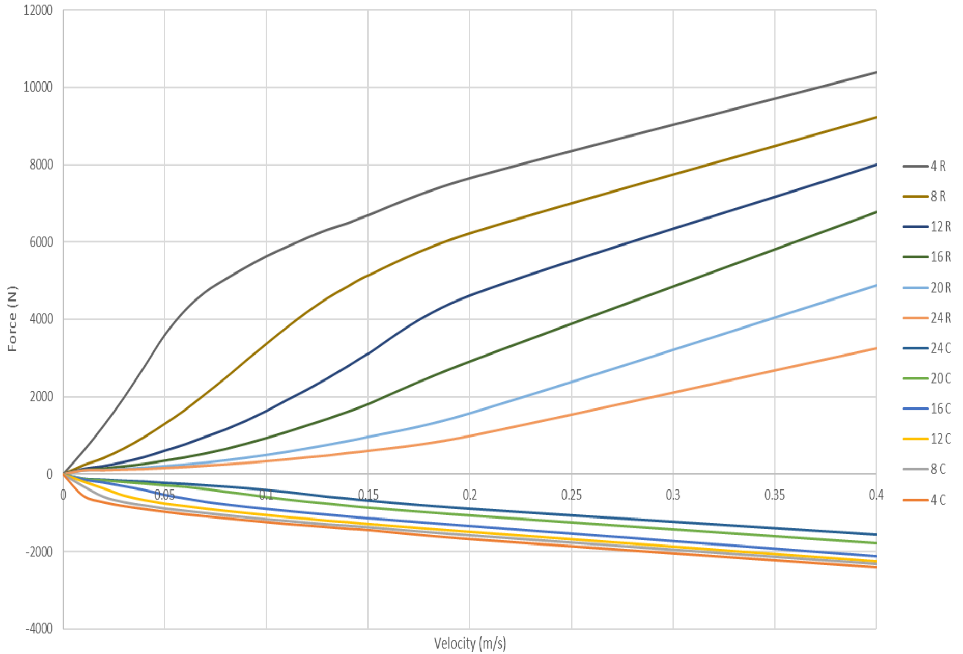
50th Anniversary CJ Rear Damper Curves
